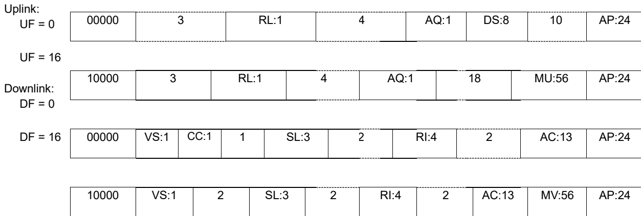
Figure 4-1. Surveillance and communication formats used by ACAS
