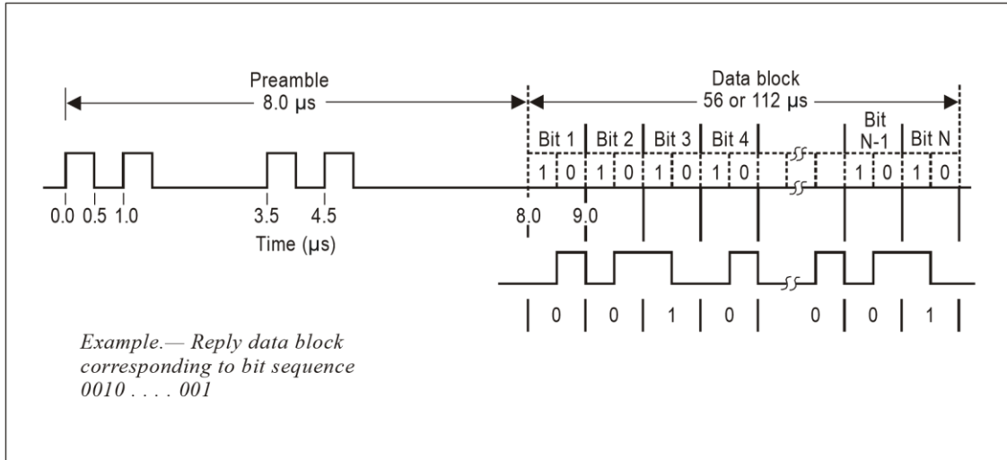
Figure 3-6. Mode S reply
