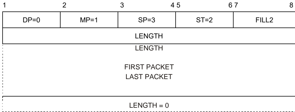
Figure 5-20. MULTIPLEX packet
