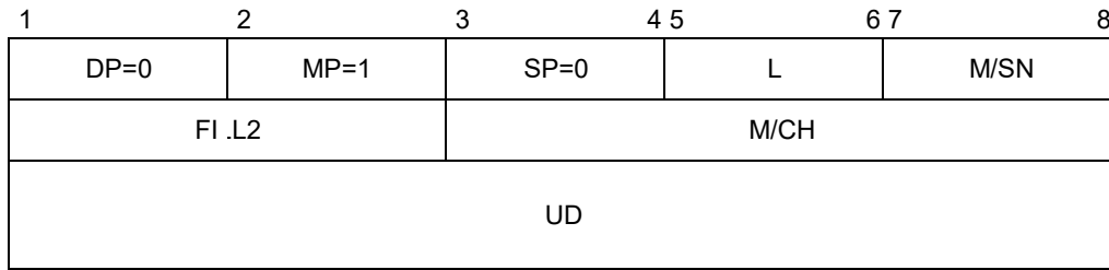
Figure 5-22. LONG FORM MSP packet
