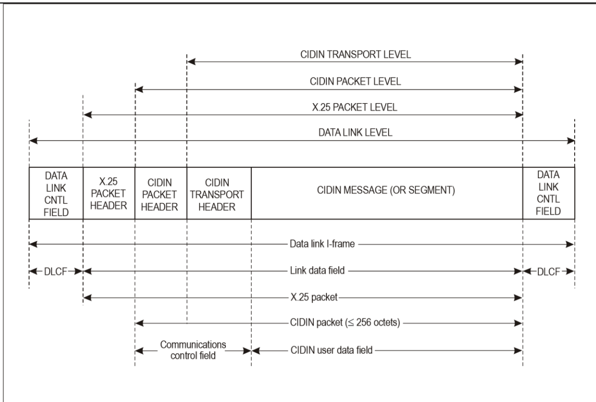
Figure 8-2. CIDIN terminology
