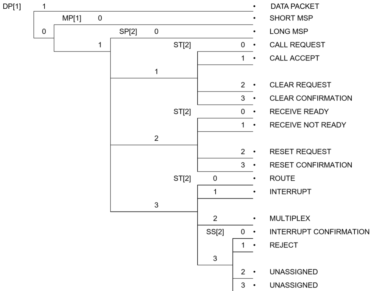
Figure 5-23. Control fields used in MODE S packets
