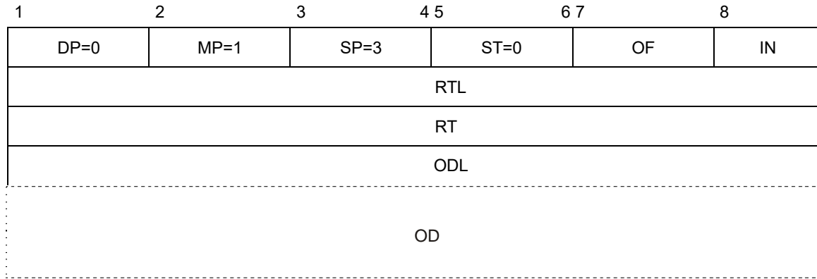
Figure 5-19. ROUTE packet
