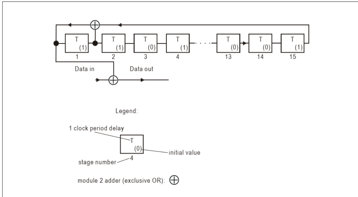
Figure 6-2. PN-generator for bit scrambling sequence
